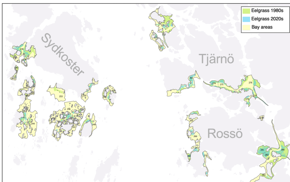
Figur 2.2 The map shows an example of eelgrass loss within 30 bay areas in northern Bohuslän since the 1980s (from Moksnes and Bergström 2025).
