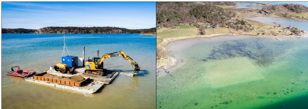
Figure 5.9. Sand capping at Lilla Askerön in March 2021 using an excavator on a floating barge anchored in the sediment with legs. The small barge in the foreground is used to transport the sand to the excavator. To the right is the one-hectare sand-covered area before eelgrass was planted.
