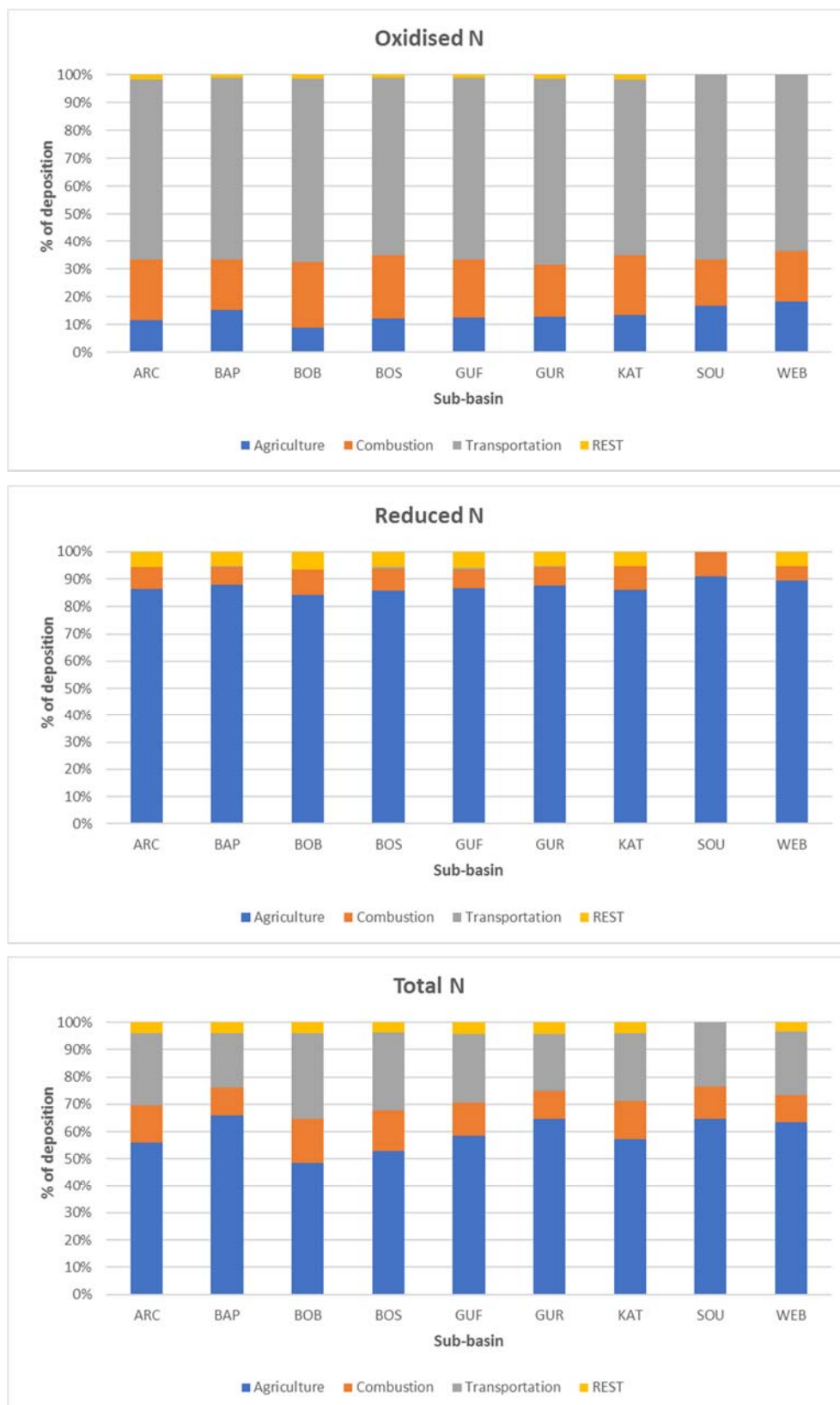
Fig. 3.12. The relative contributions from Lithuania to oxidised, reduced and total nitrogen deposition to individual Baltic Sea sub-basins in 2014. Units: % of total deposition from Lithuania.
