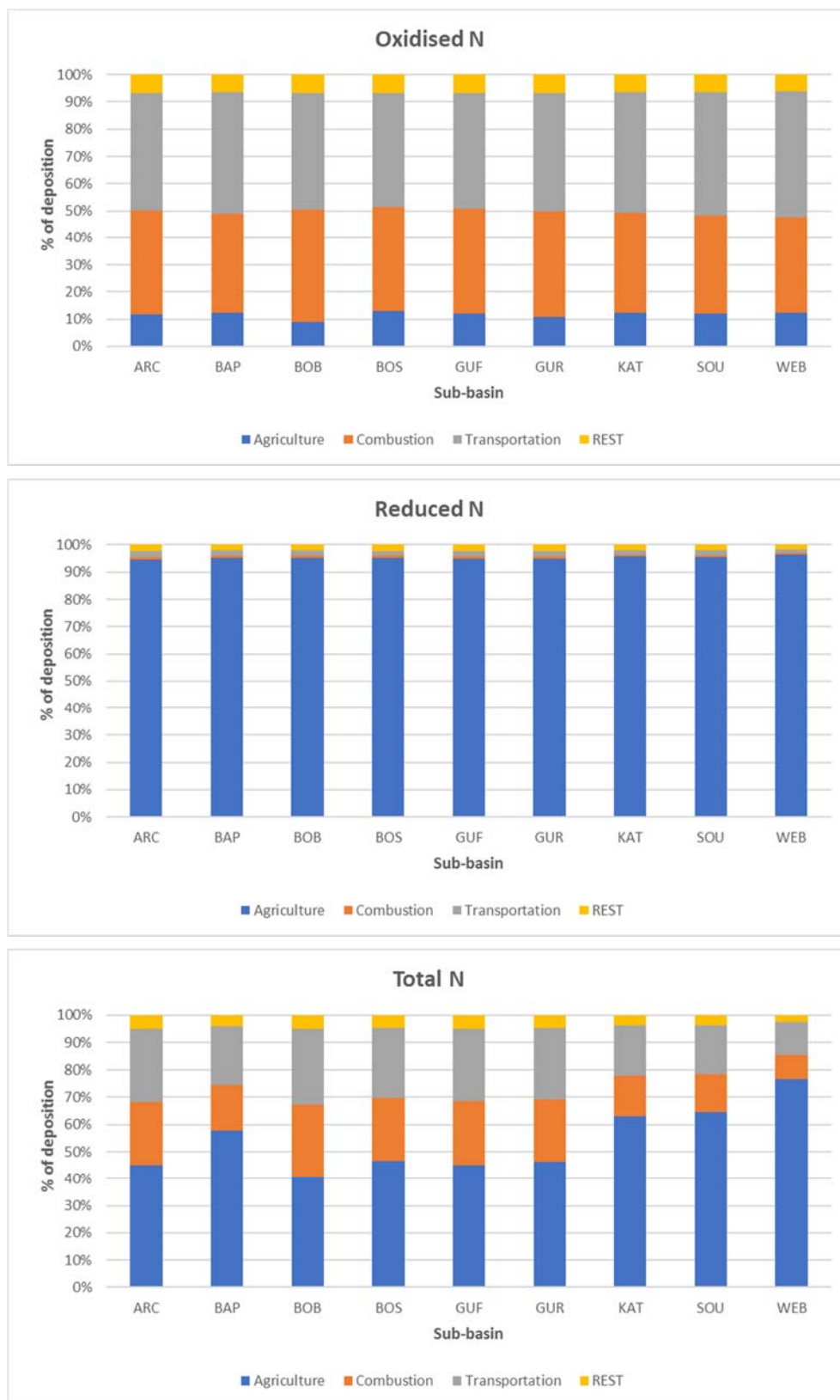
Fig. 3.8. The relative contributions from Germany to oxidised, reduced and total nitrogen deposition to individual Baltic Sea sub-basins in 2014. Units: % of total deposition from Germany.
